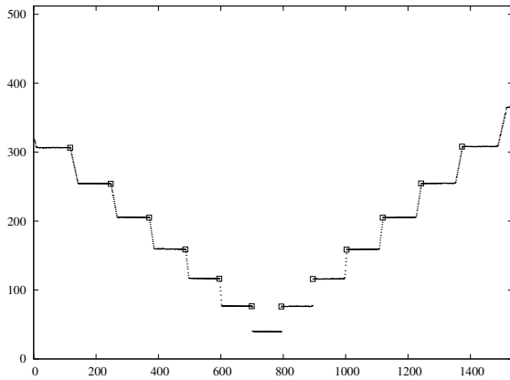
Fig. 5. Typical Point Detection Result
