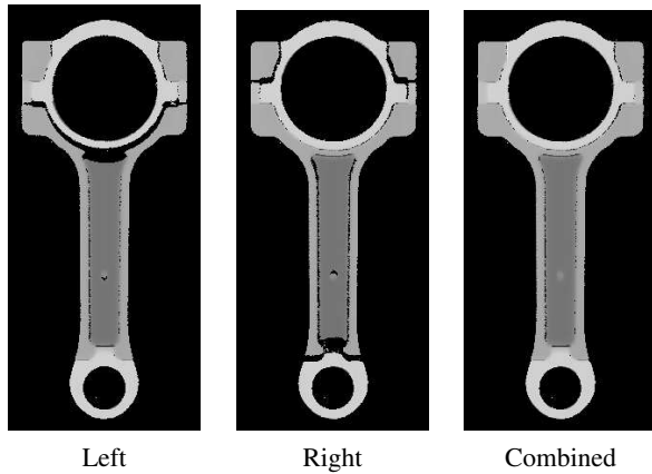
Fig. 6. Occlusion Reduction for Connecting Rod
